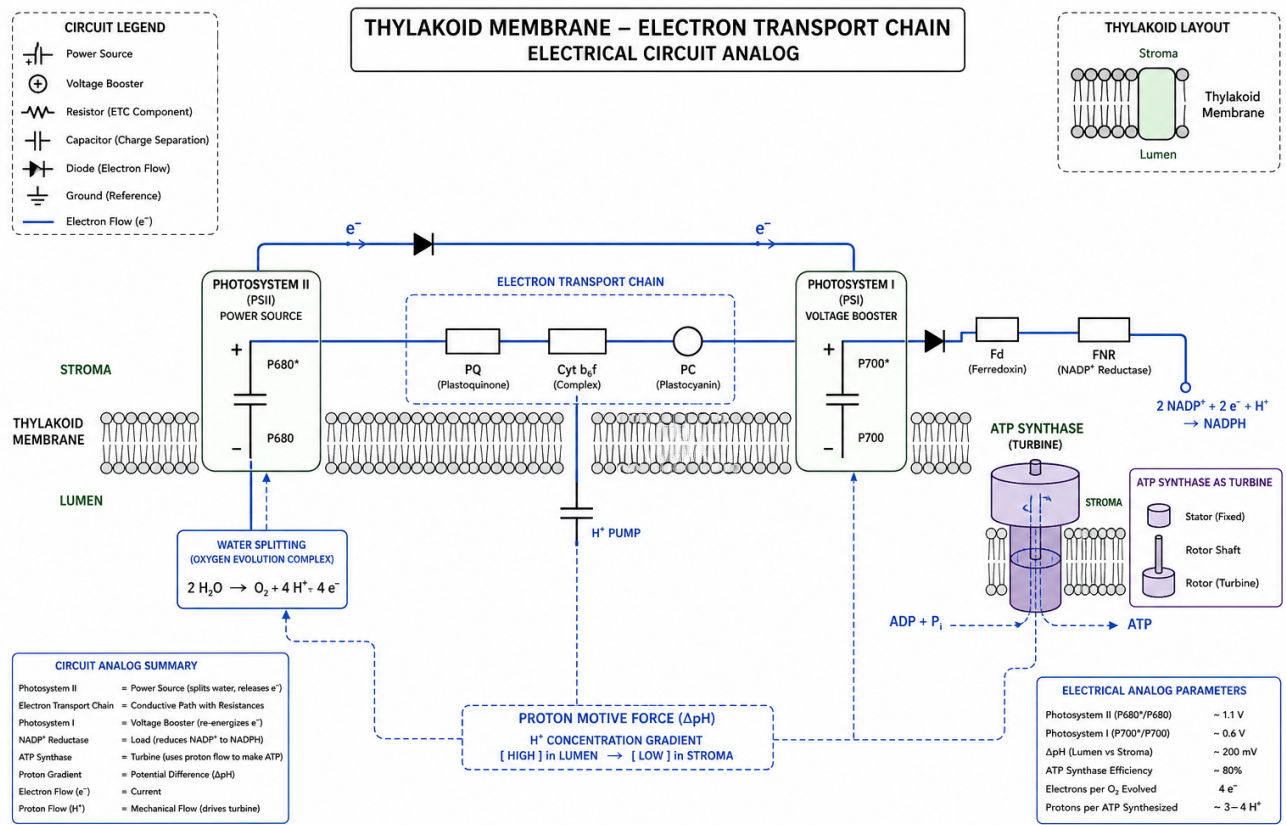
Fig. 2. The electron transport chain viewed as a biological circuit. Electrons flow from water to NADP ^+ via two solar-powered voltage boosts, while protons are pumped across the membrane to drive the ATP synthase motor. Image generated using ChatGPT AI.
